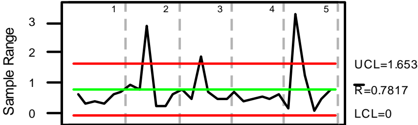
R Chart by MAT
