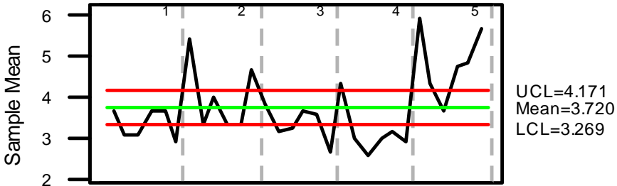
Xbar Chart by MAT
